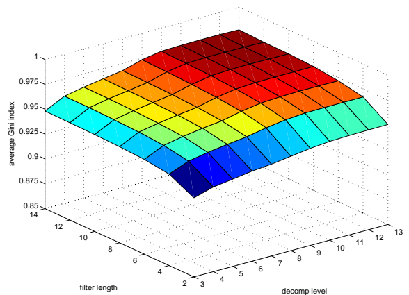
Fig. 8. Sparsity for wavelet packet decomposition using Daubechies wavelets of length 2, 4, 6, 8, 10, 12, 14 and decomposition level 3 through 13. Binary tree selection using greedy selection method.
