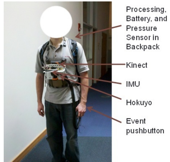
Fig. 2. A user carrying our prototype human-portable mapping system
