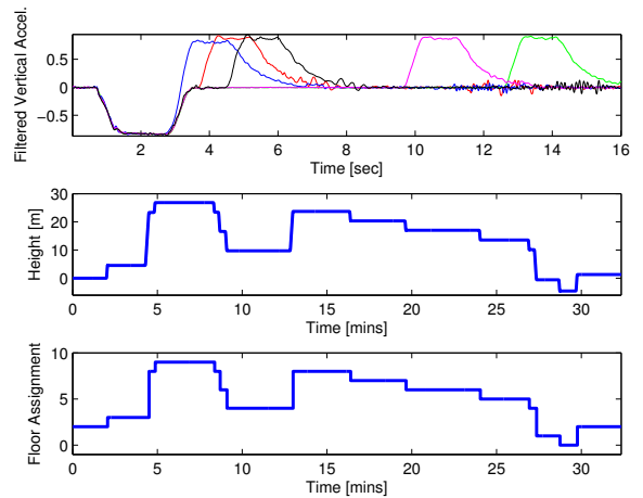
Fig. 7. Top: Filtered IMU Z-component for 5 elevator rides. Middle: Height can be estimated by integrating the elapsed time between the characteristic accelerations and decelerations. Bottom: Using this approach we successfully estimated the floor transitions across a 35 minute experiment across 10 floors - beginning and ending on Floor 2 of MIT's Stata Center.
