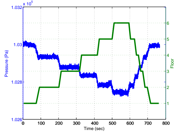
Fig. 6. The raw pressure readings (blue) are processed using a Gaussian mixture model to detect floors (green).
