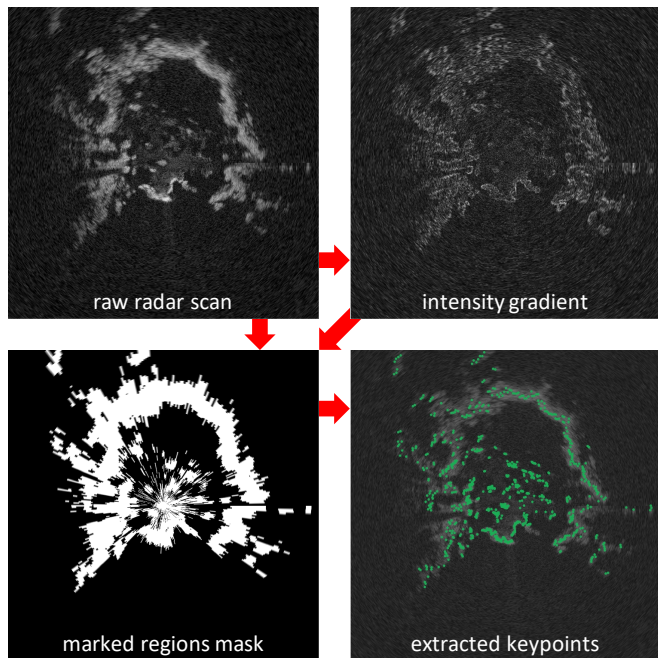
Fig. 3: Visualization of our keypoint extraction approach operating in a forest in Iceland. From the 250 \times 250 m radar scan (top left) and its intensity gradient (top right), important regions in the scan are identified. Those marked (bottom left), the number of which is capped by the only tunable parameter \ell_{\max} , are used to produce a keypoint set (bottom right) that captures the scene structure while minimizing redundant keypoints.
