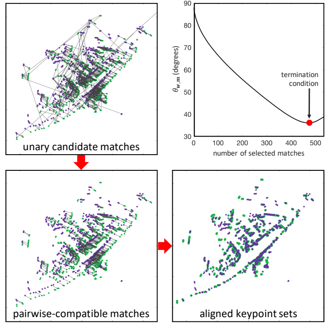
Fig. 4: Visualization of our data association approach operating in Warwick, UK. It first proposes unary matches using feature descriptors (top left), then uses pairwise relationships to identify mutually consistent matches (bottom left). Our method approximates the solution to an NP-hard problem using a greedy algorithm, for which the termination condition is visualized on the top right. The final alignment (bottom right) shows the robustness to noise.
