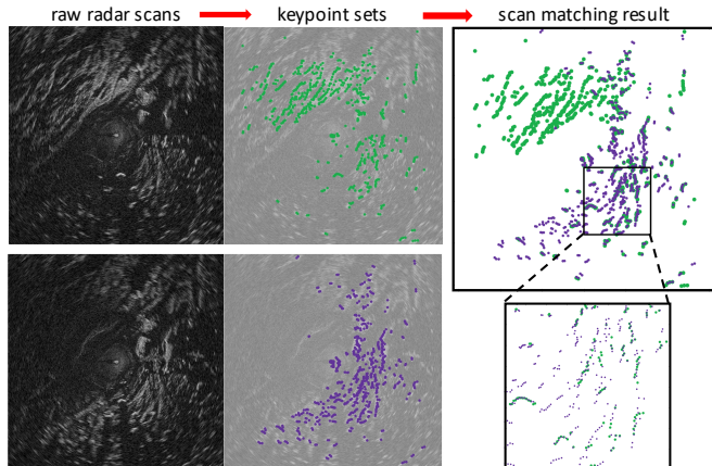
Fig. 1: Demonstration of our one-parameter, radar-only odometry pipeline performing scan matching in a challenging scenario with no motion prior. On the left are two consecutive radar scans, which are 250 \times 250 m and taken 0.25 seconds apart while driving over uneven open terrain in Iceland. The keypoints extracted by our algorithm are shown in green and purple, and the alignment proposed by our data association algorithm is visualized on the right. Precise scan matching is achieved despite radar’s high levels of measurement noise as well as significant appearance changes.
